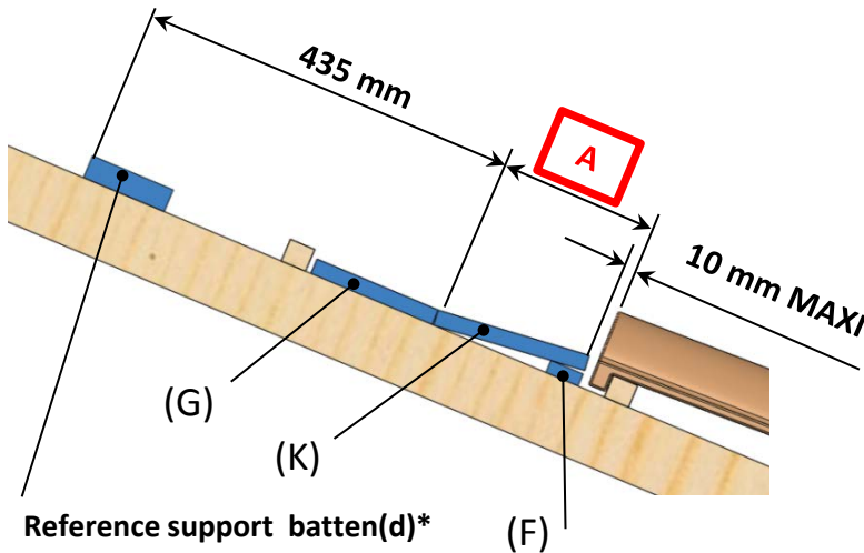
The bottom flashing batten and the bottom flashing itself will have to be 2 tiles longer on each side of the PV field.
