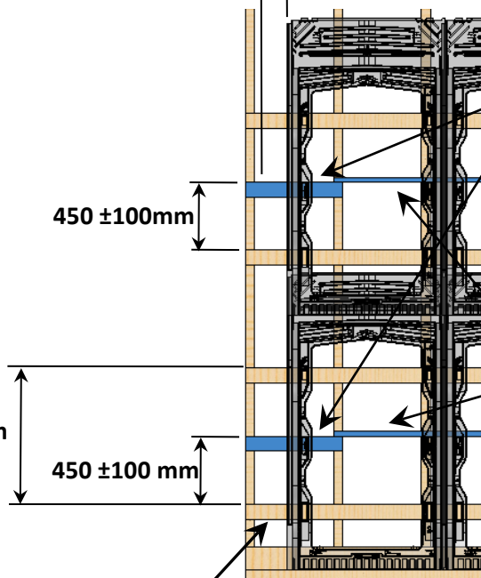
Reference support batten (view without the tiles batten)
