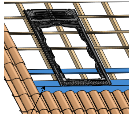
The bottom flashing batten and the bottom flashing itself will have to be 2 tiles longer on each side of the PV field.
